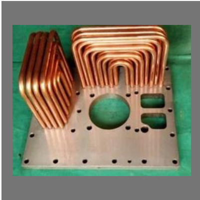
Tanabe Air Compressor Cooler Plate
